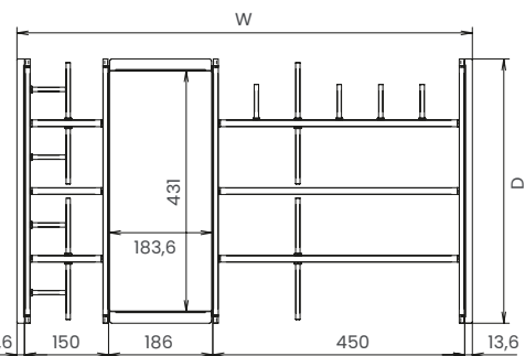
Tandembox | F 19
