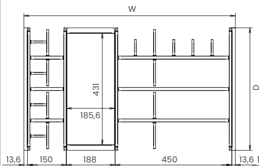
Tandembox | F 18
